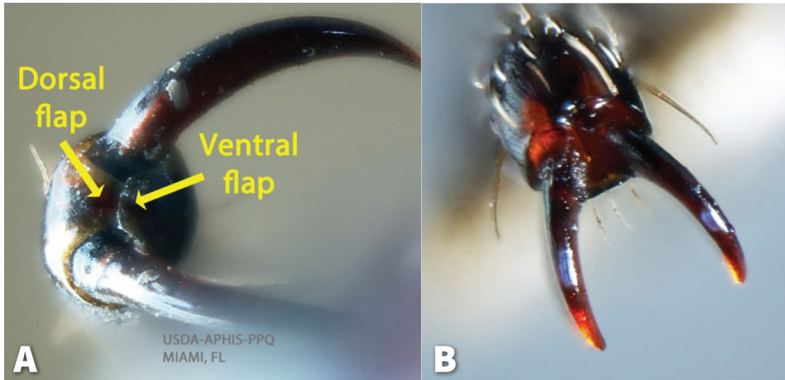
Figure 20. Tarsal claw characteristics: flaps between tarsal claws are present in (a) Dryophthoridae and absent in (b) Curculionidae . © USDA/APHIS/PPG/Charles Brodel
