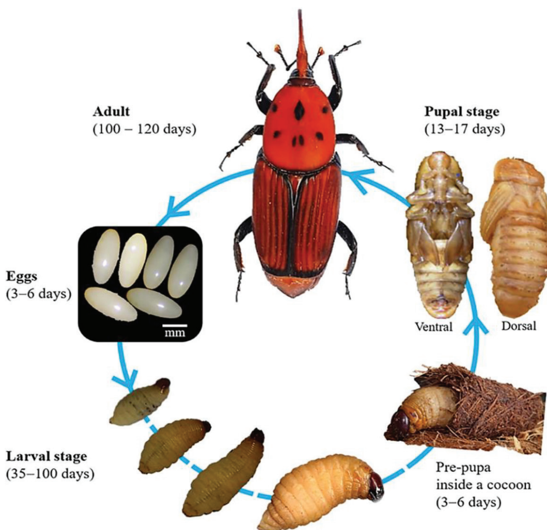
Figure 14. Red palm weevil life cycle. © CABI
