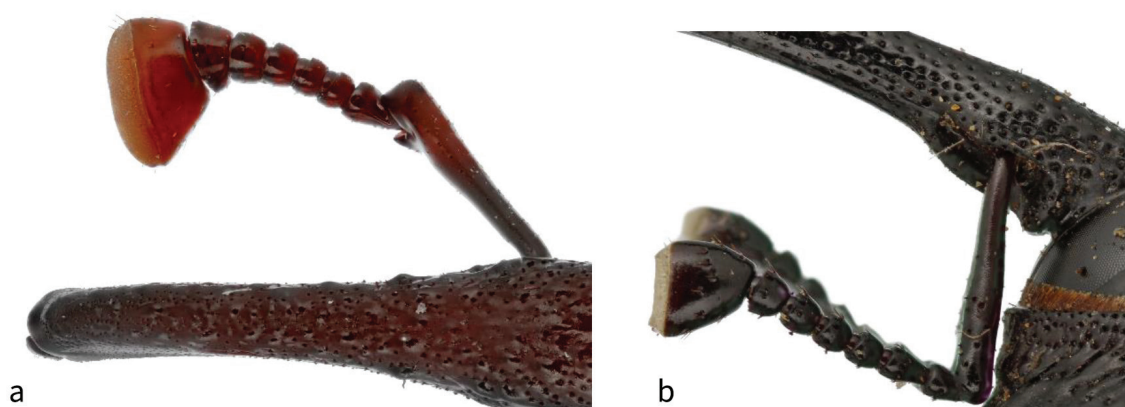
Figure 23. Antennae shape: (a) Rhynchophorus antennae have a wide antennal club; (b) Scyphophorus have a longer antennal club. © USDA-APHIS-PPQ-ITP/Hanna Royals
